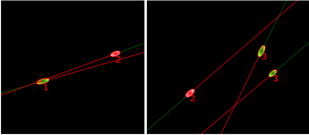
Figure 10. False classification with thumb and ring-finger / little-finger. An ellipse depicts a touch contact, the lines depicts the orientation and the numbers denotes the recognized hand ids.
